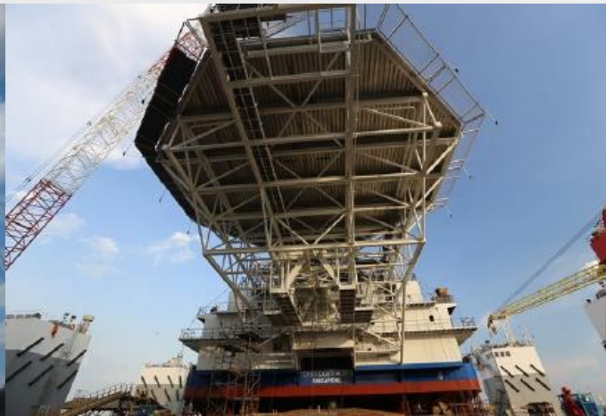
H1018 Helipad/Accommodation/Machinery installation. Sea Trial due in July
