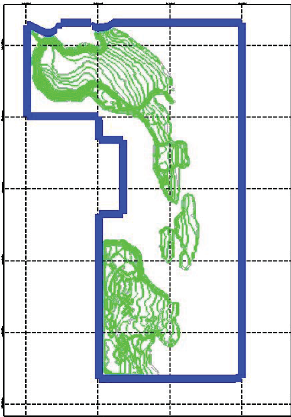
Figure 9:6 Final Pit Design – Kusan Girimulya Pits
