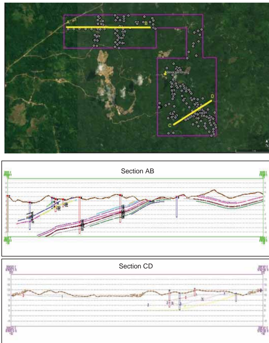
Figure 4:3 TKS Ampah – Coal Seam Cross Section
