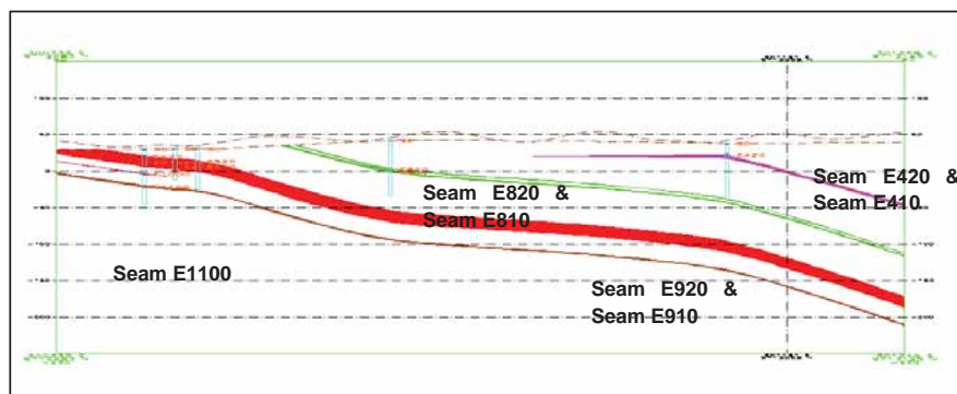
Figure 4:3 BL Block - Typical Cross Section
