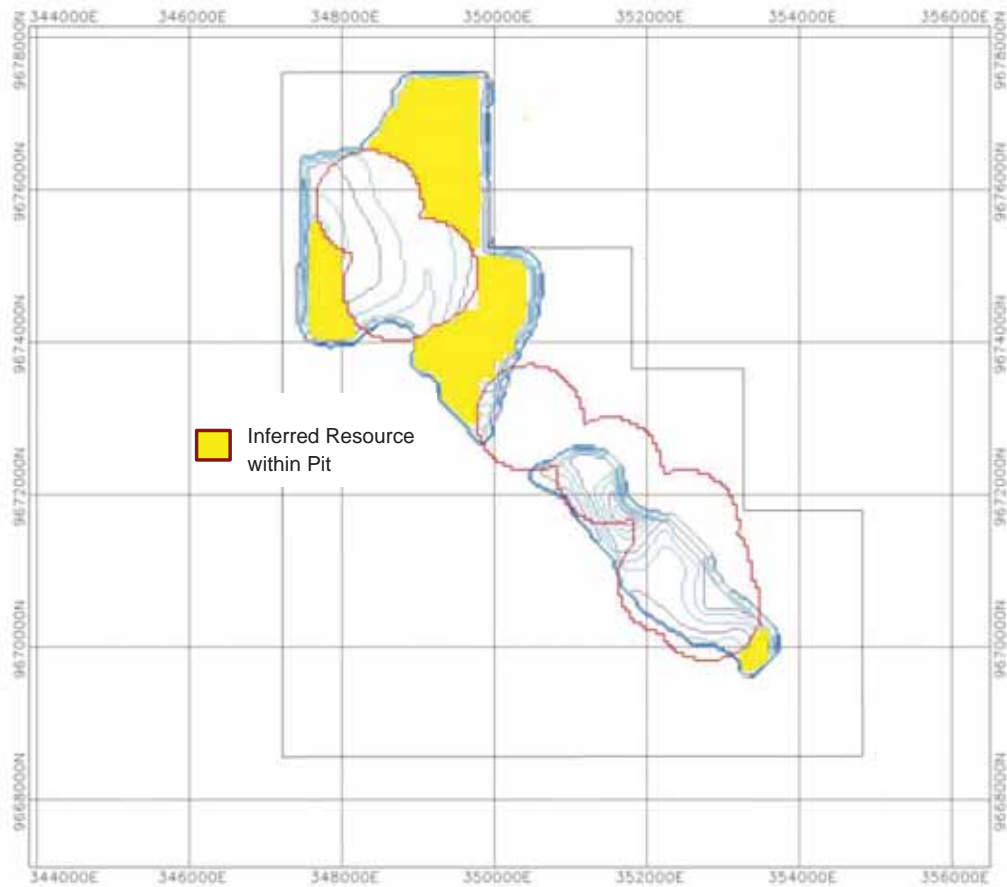
Figure 7:7 WRL Pit with P14U Indicated Resource Polygon
