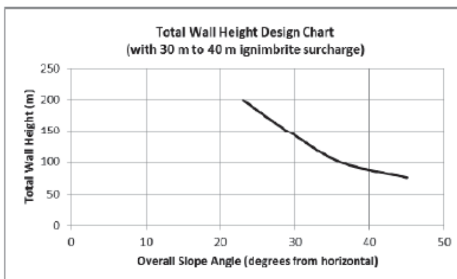
Figure 7:2 Geo-tech Recommendations
