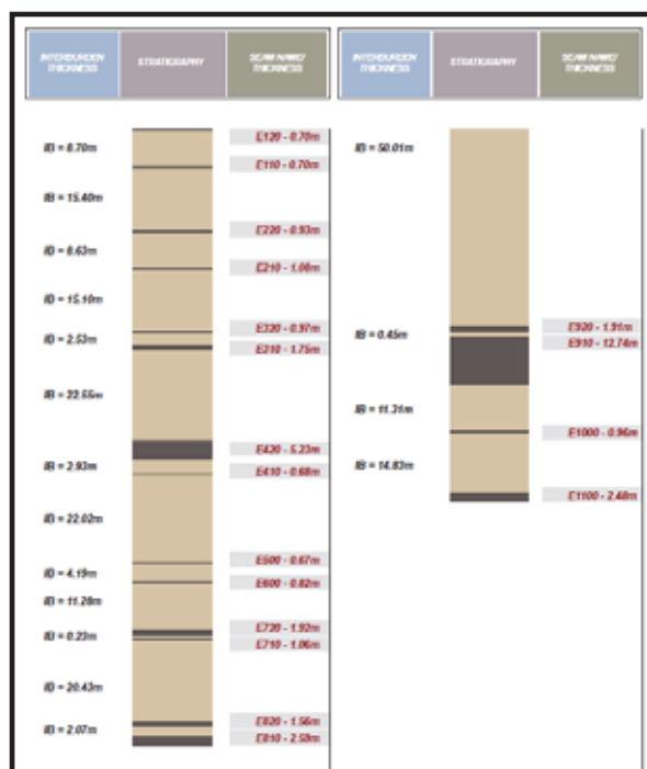
Figure 4:4 BL Block - Generalised Stratigraphic Column
