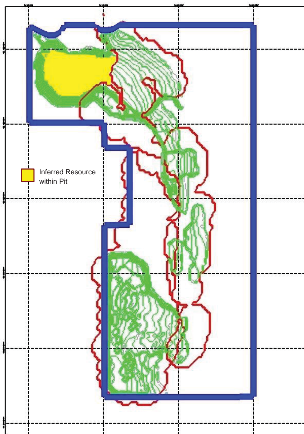
Figure 9:7 KG Pit with E1U2 & BL2U Indicated Polygons
