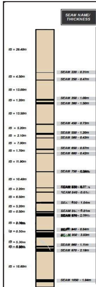
Figure 4:2 ML Block - Generalised Stratigraphic Column
