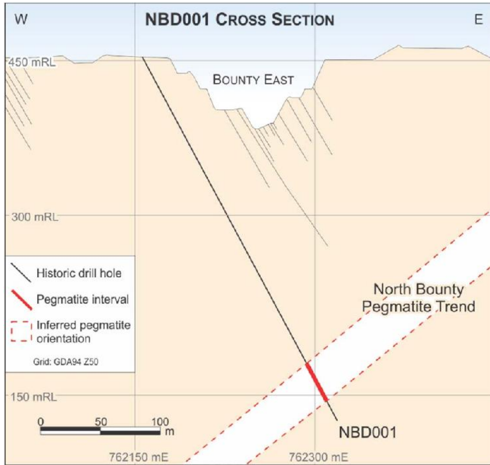
Figure 3: NBD001 Cross section.
