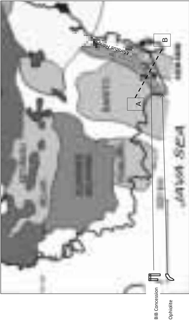
Figure 4:2 Regional Geological Setting
