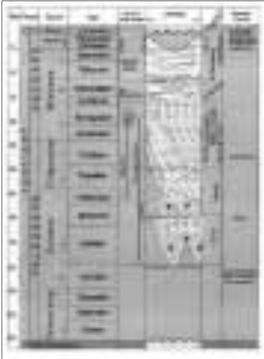
Figure 4:1 Generalised Stratigraphy of the South Sumatra Basin
