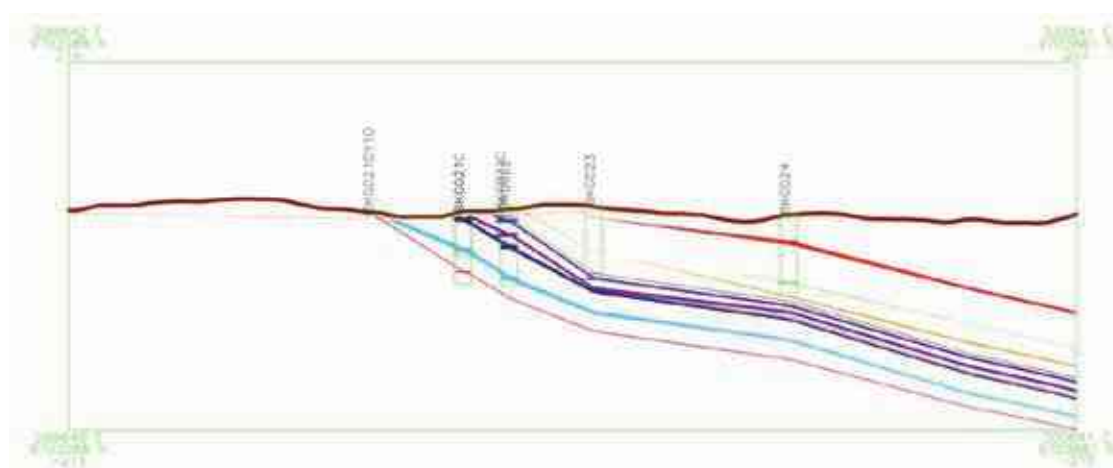
Figure 4:6 BK Block - Typical NE-SW Cross Section
