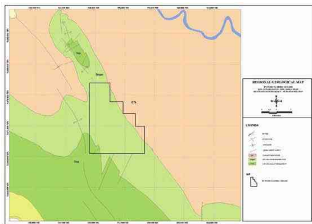
Figure 4:2 Local geological map of the WRL concession area
