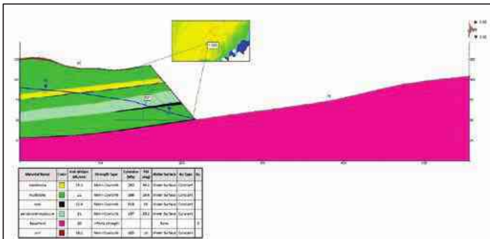
Figure 9:3 Geotechnical simulation for slope of 50°, Safety factor of 1.46
