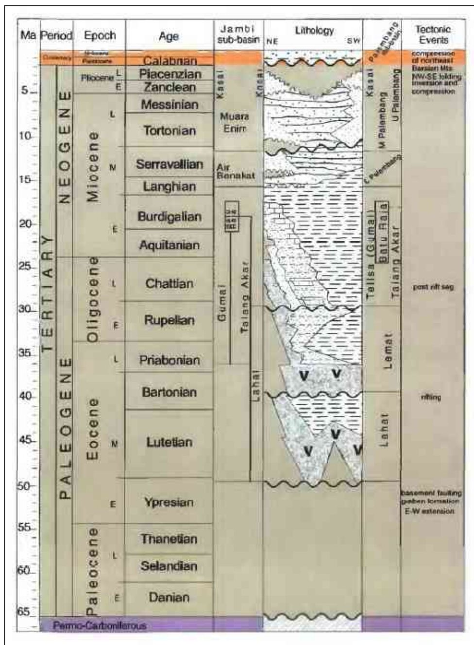
Figure 4:1 Generalised Stratigraphy of the South Sumatra Basin
