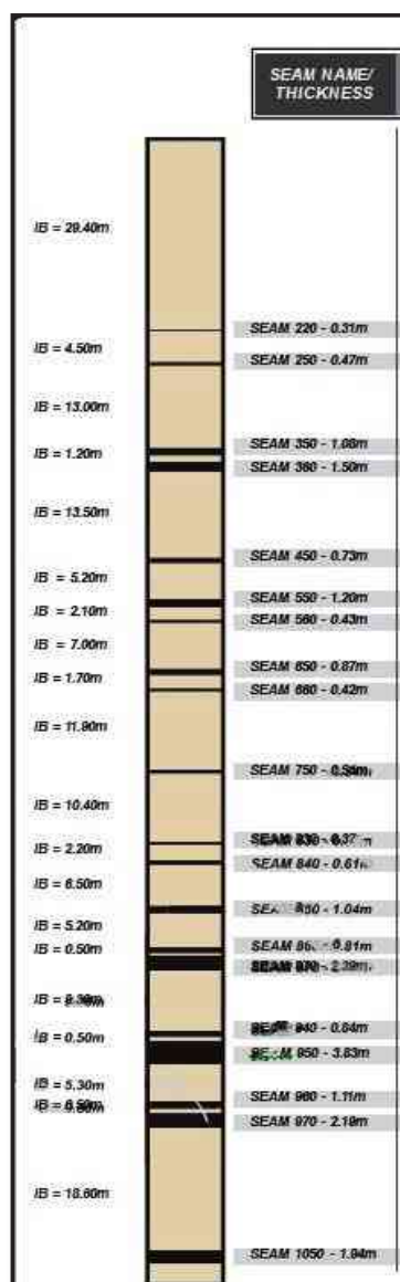
Figure 4:3 ML Block - Generalised Stratigraphic Column
