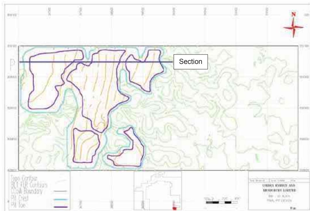
Figure 9:17 Final Pit Design – Sebamban South (SS Pit)
