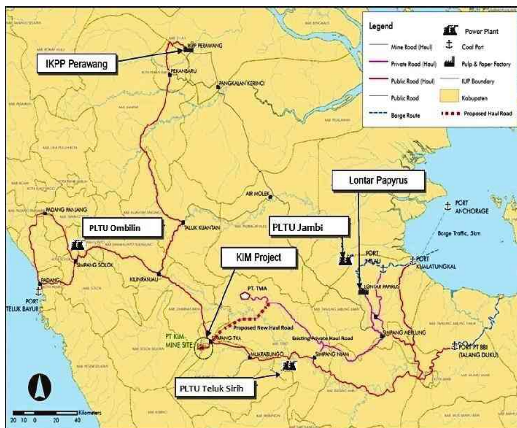
Figure 8:5 Current and Proposed Coal Logistics, KIM Project
