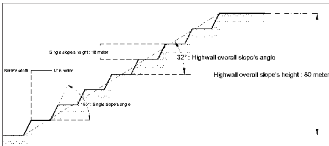
Figure 9:1 Pit Geometry Recommendation, Geotechnical Study
