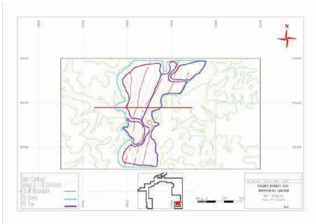
Figure 9:19 Final Pit Design – Sebamban North (SN Pit)
