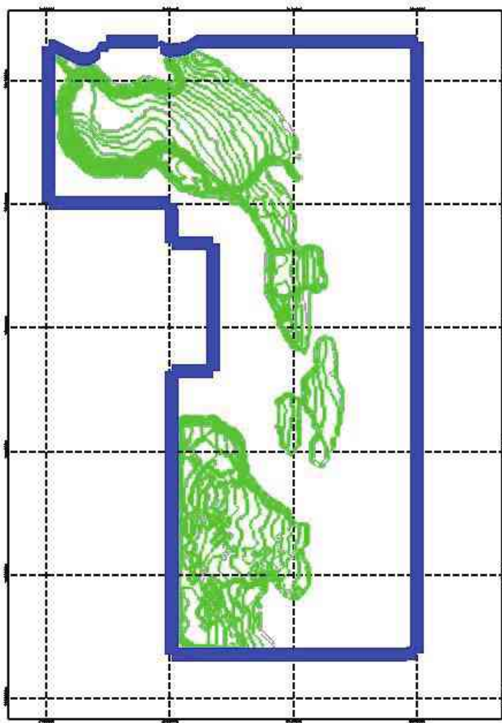
Figure 9:11 Final Pit Design – Kusan Girimulya Pits
