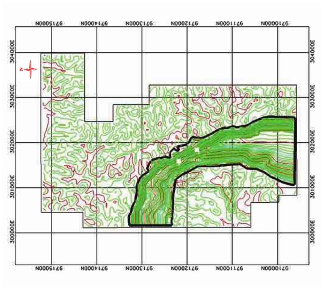
Figure 8:13 Final Pit Design, Belani
