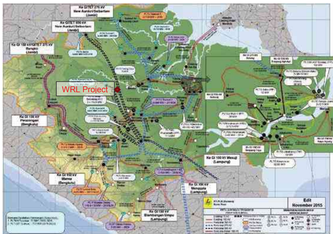
Figure 9:5 Planned Electricity Network, South Sumatra
