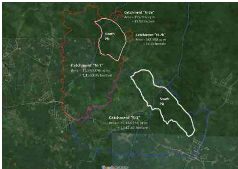
Figure 9:2 Catchment Area from Hydrology Study
