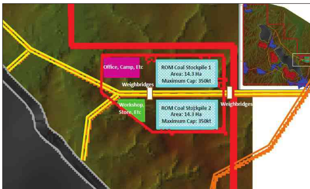
Figure 9:4 Proposed ROM Layout
