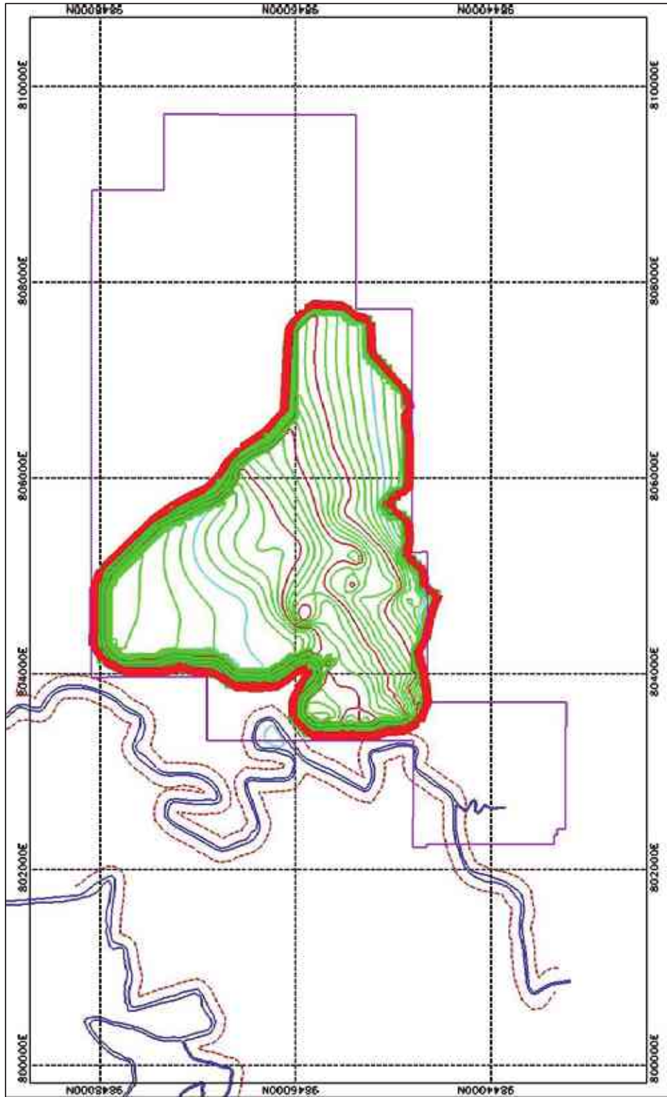
Figure 8:10 Selected Optimiser Pit shell - KIM East
