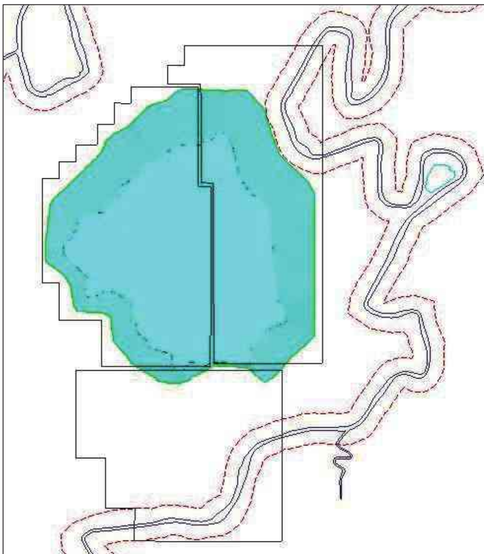
Figure 8:7 Final Pit Design - KIM West
