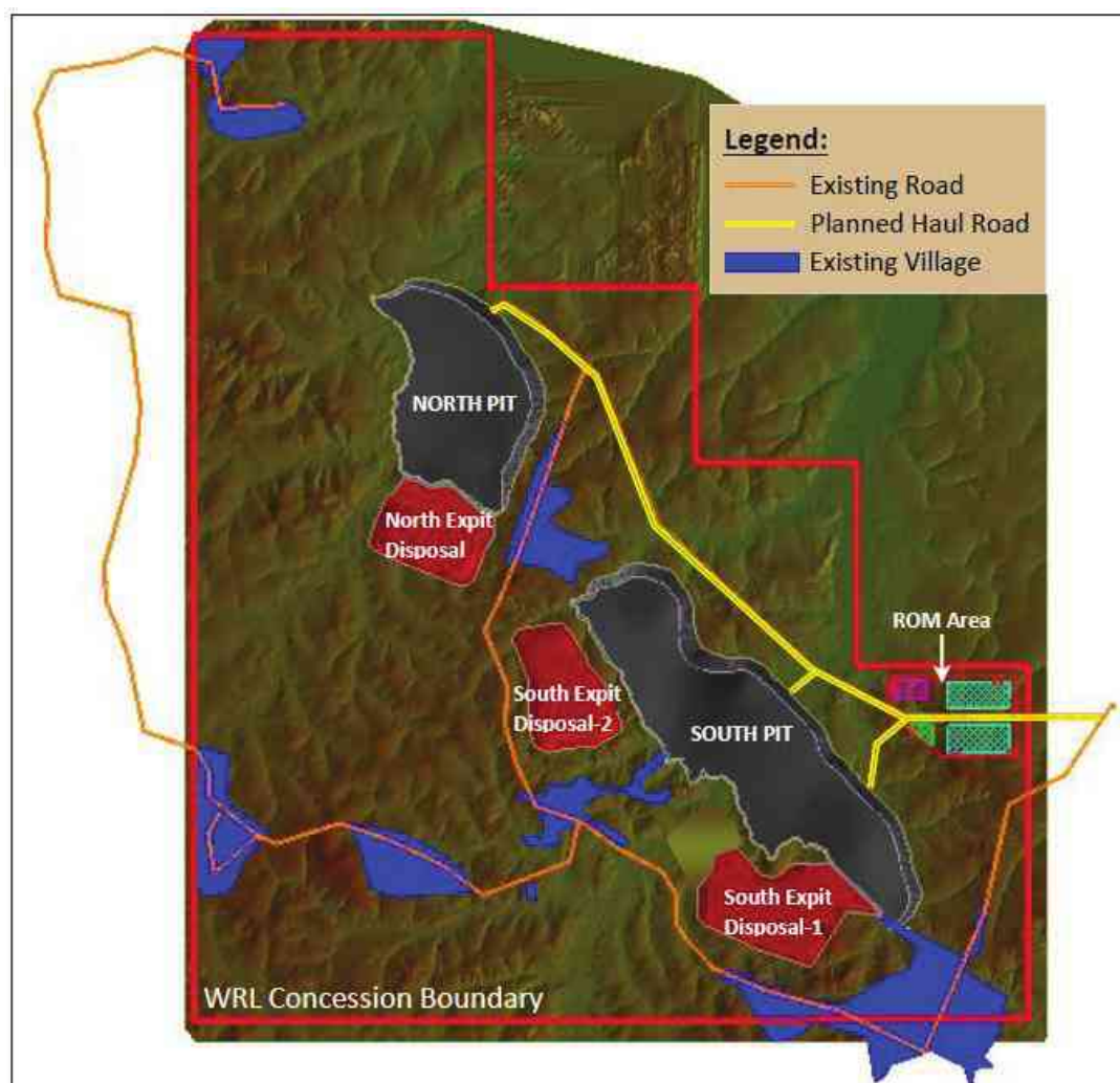
Figure 9:3 Proposed Mining Infrastructure and Facilities
