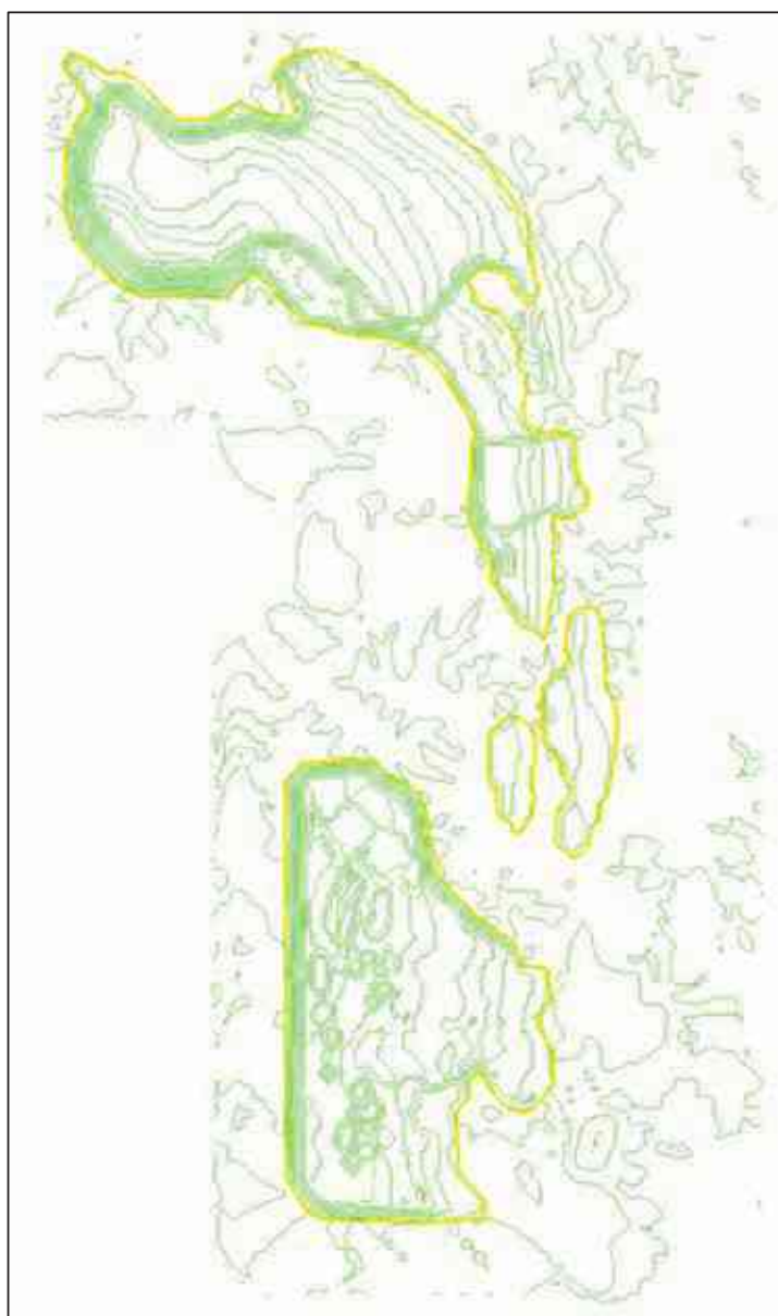
Figure 9:6 Pit shell selection & Final Pit Design – KG Block
