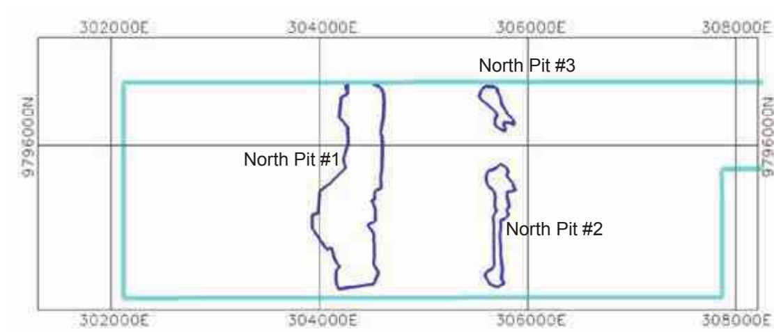
Figure 9:5 Pit Selection – TKS Ampah North Section
