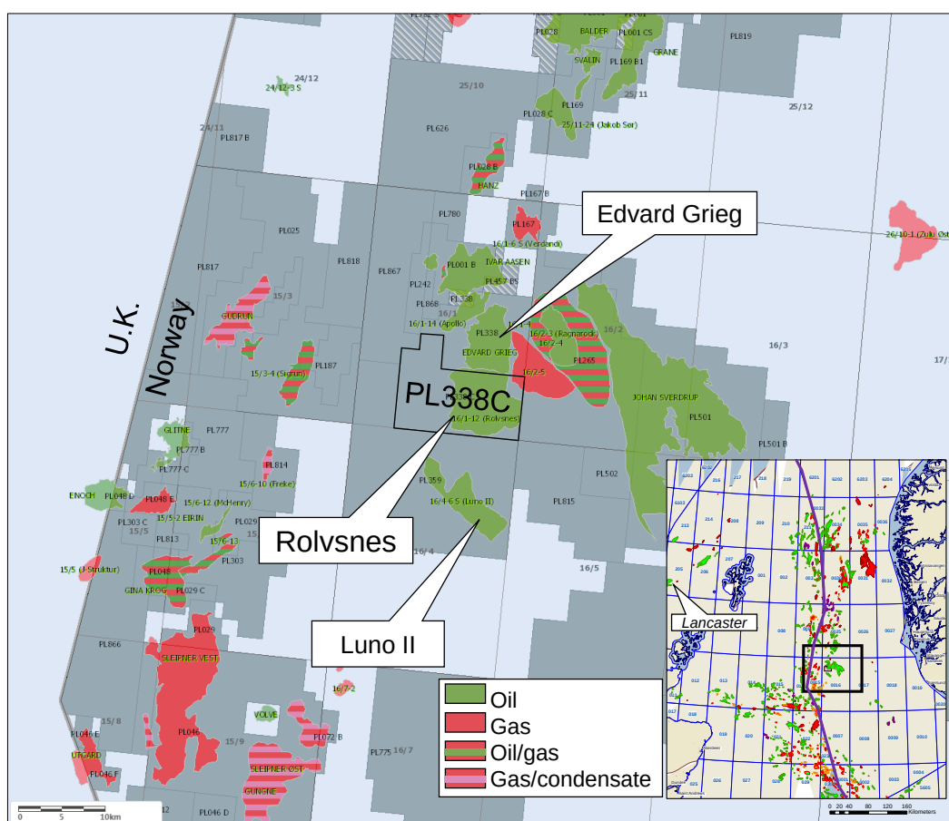
Figure 1: Rolvsnes Discovery Location Map
