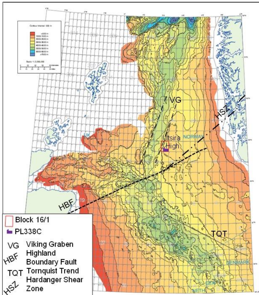
Figure 2: Regional Depth Structure to BCU with Tectonic Fabric Overlain
