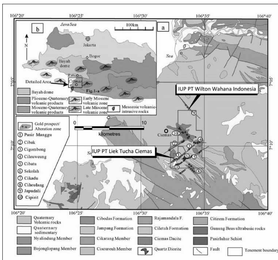
Diagram 1 : Geology of the Ciemas Gold Project
