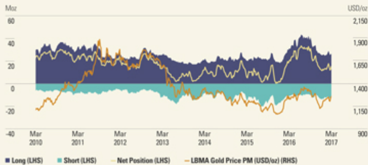
Figure 6: COMEX Positioning
