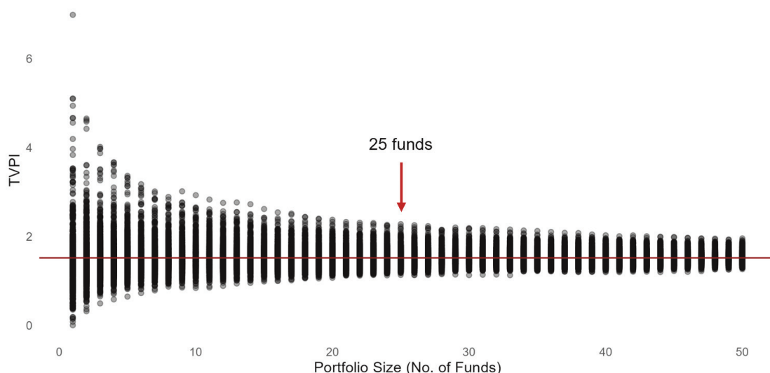
Figure 4: TVPI versus portfolio size for simulated portfolios
