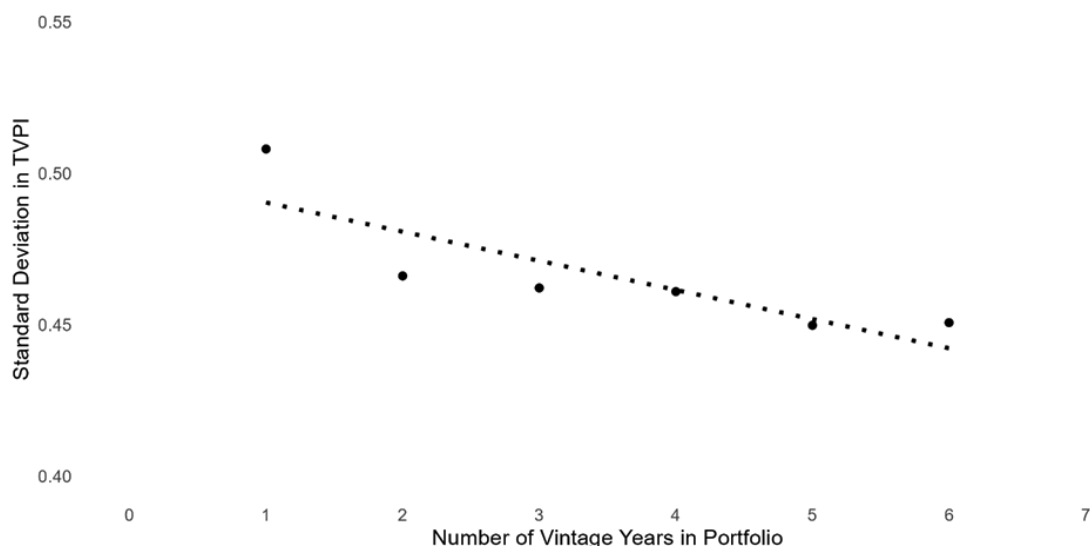
Figure 6: Standard deviation in TVPI versus number of vintage years in simulated portfolios
