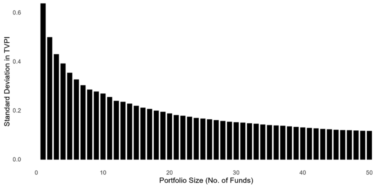
Figure 5: Standard deviation in TVPI versus portfolio size for simulated portfolios
