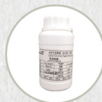
Sodium hydroxide
